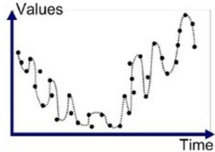
Overfitted
