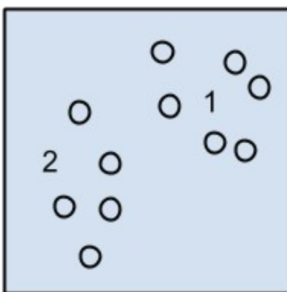
Clustering Algorithms
