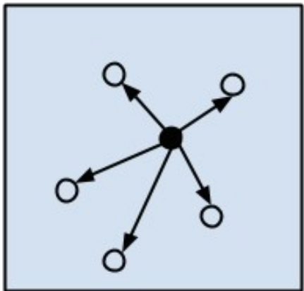
Instance-based Algorithms
