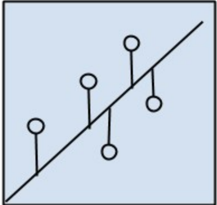
Regression Algorithms
