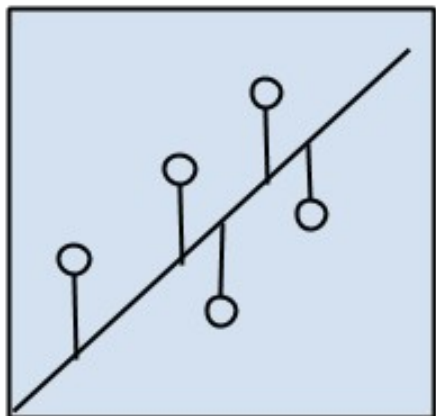
Regression Algorithms
