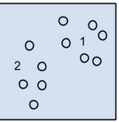
Clustering Algorithms
