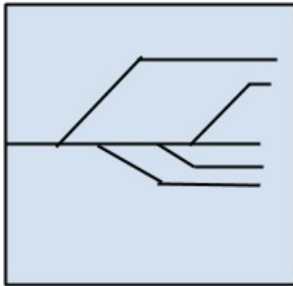
Regularization Algorithms
