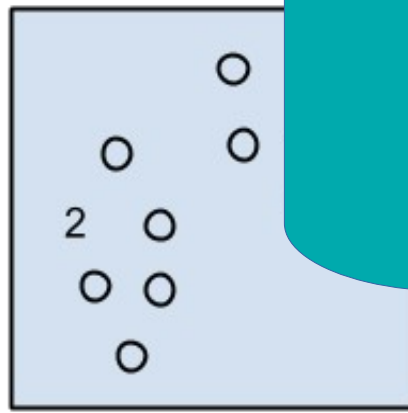
Clustering Algorithms
