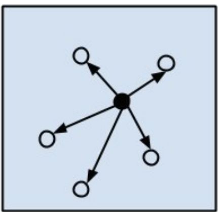
Instance-based Algorithms
