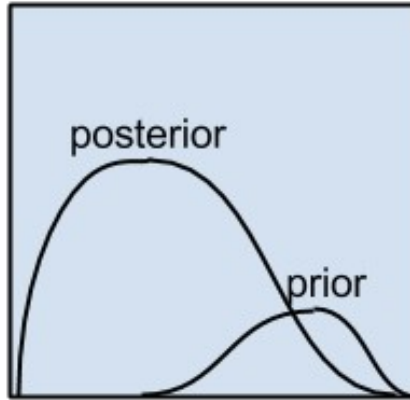
Bayesian Algorithms
