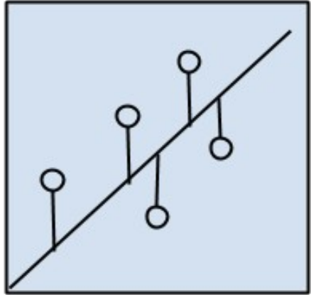
Regression Algorithms
