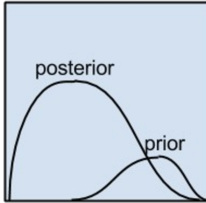
Bayesian Algorithms
