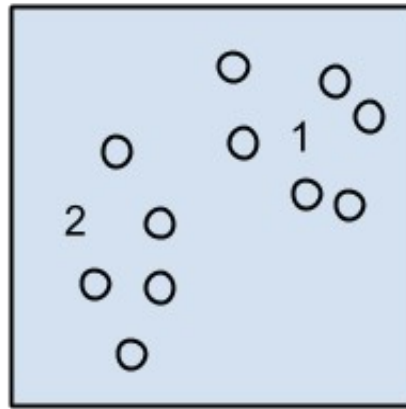
Clustering Algorithms
