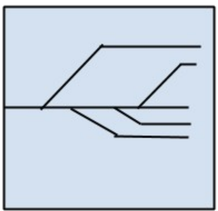
Regularization Algorithms
