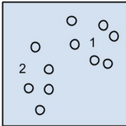
Clustering Algorithms
