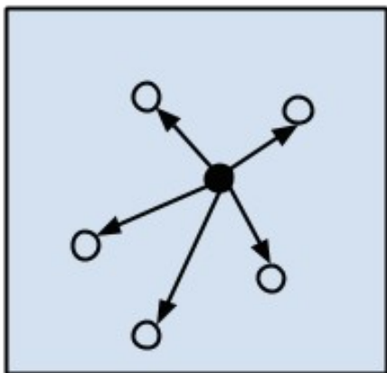
Instance-based Algorithms
