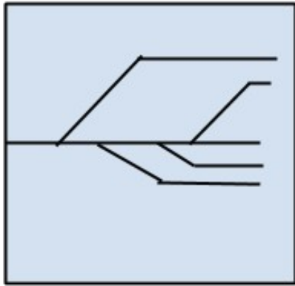
Regularization Algorithms
