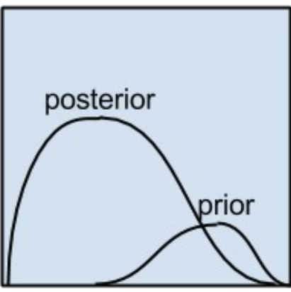
Bayesian Algorithms
