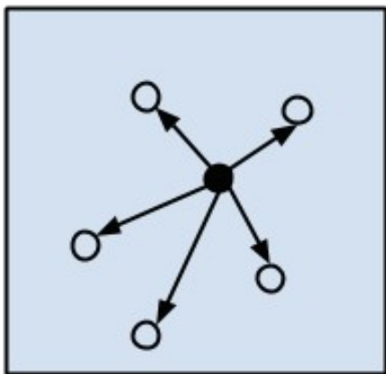
Instance-based Algorithms
