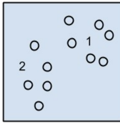
Clustering Algorithms
